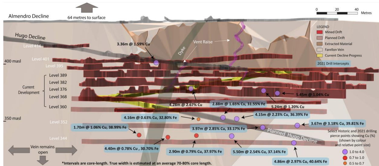
Figure 4. Farellon Mine Section
